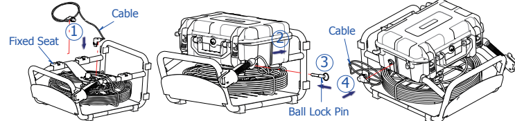
Figure 7. Install toolbox
